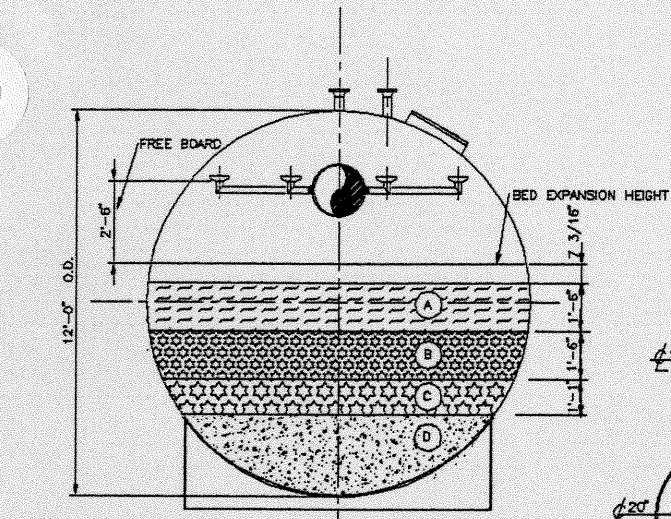
MEDIA GRADATION SCALE: 3/8"=1'-0"
